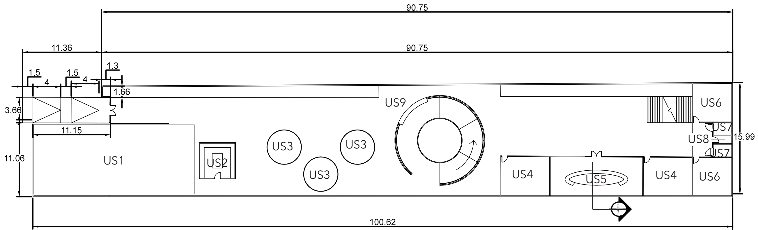
FOUNDATION PLAN OF UNDERGROUND
