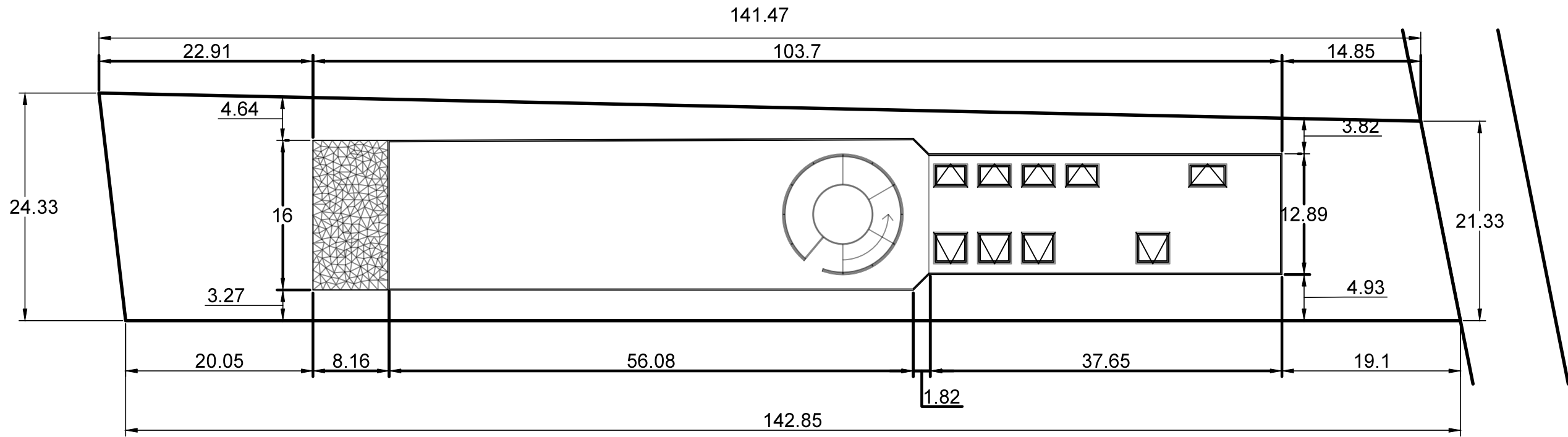
FOUNDATION PLAN ON SITE
